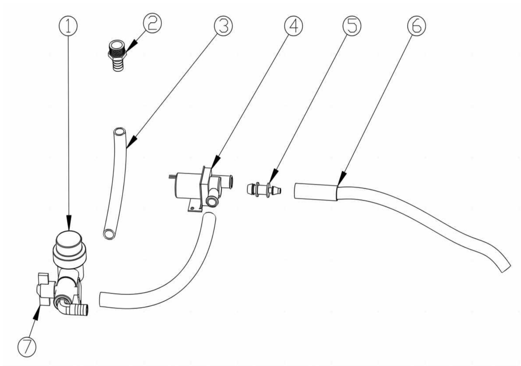
Fig. 7 -HOSE GROUP
