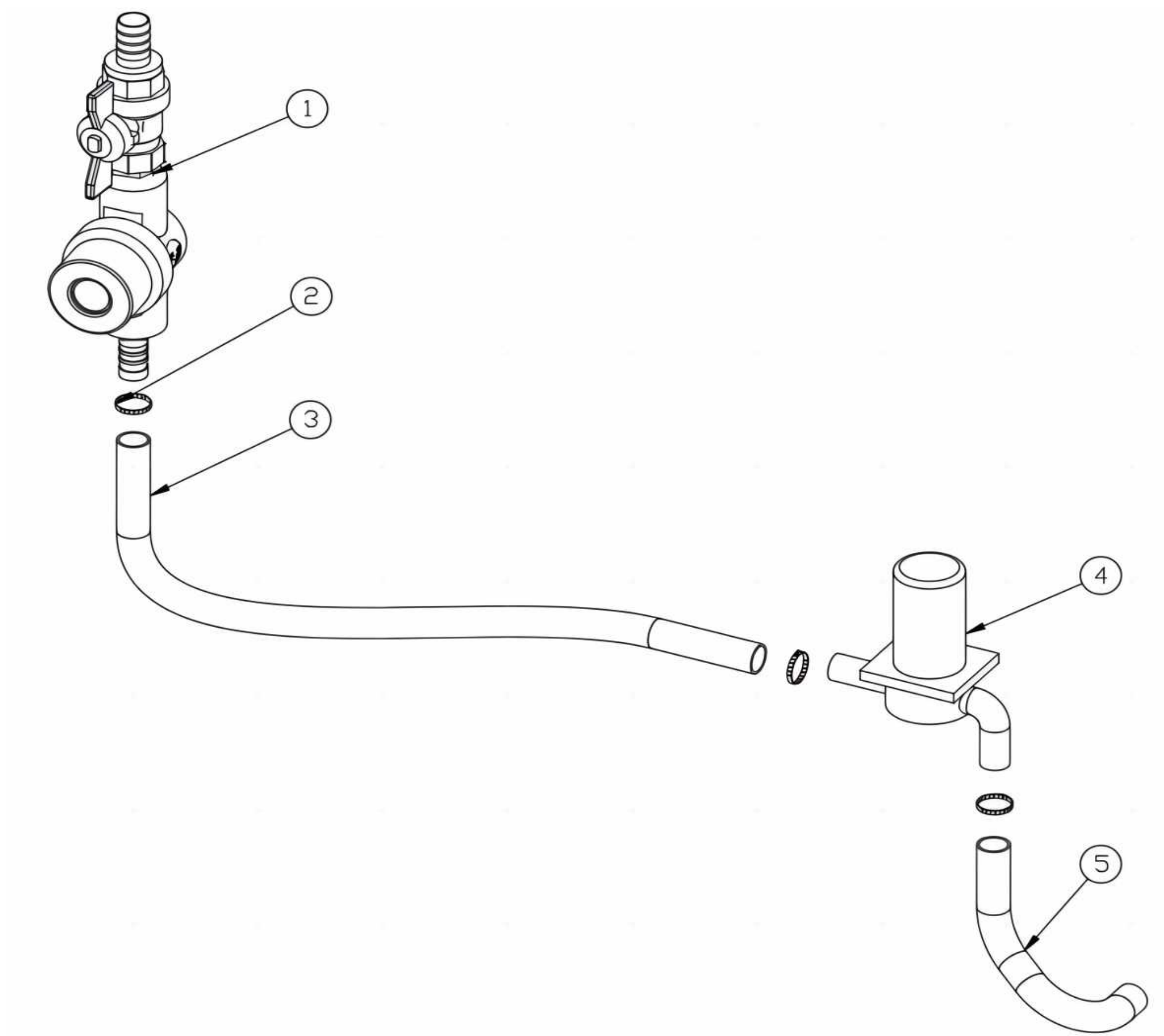
Fig. 6 -HOSE GROUP
