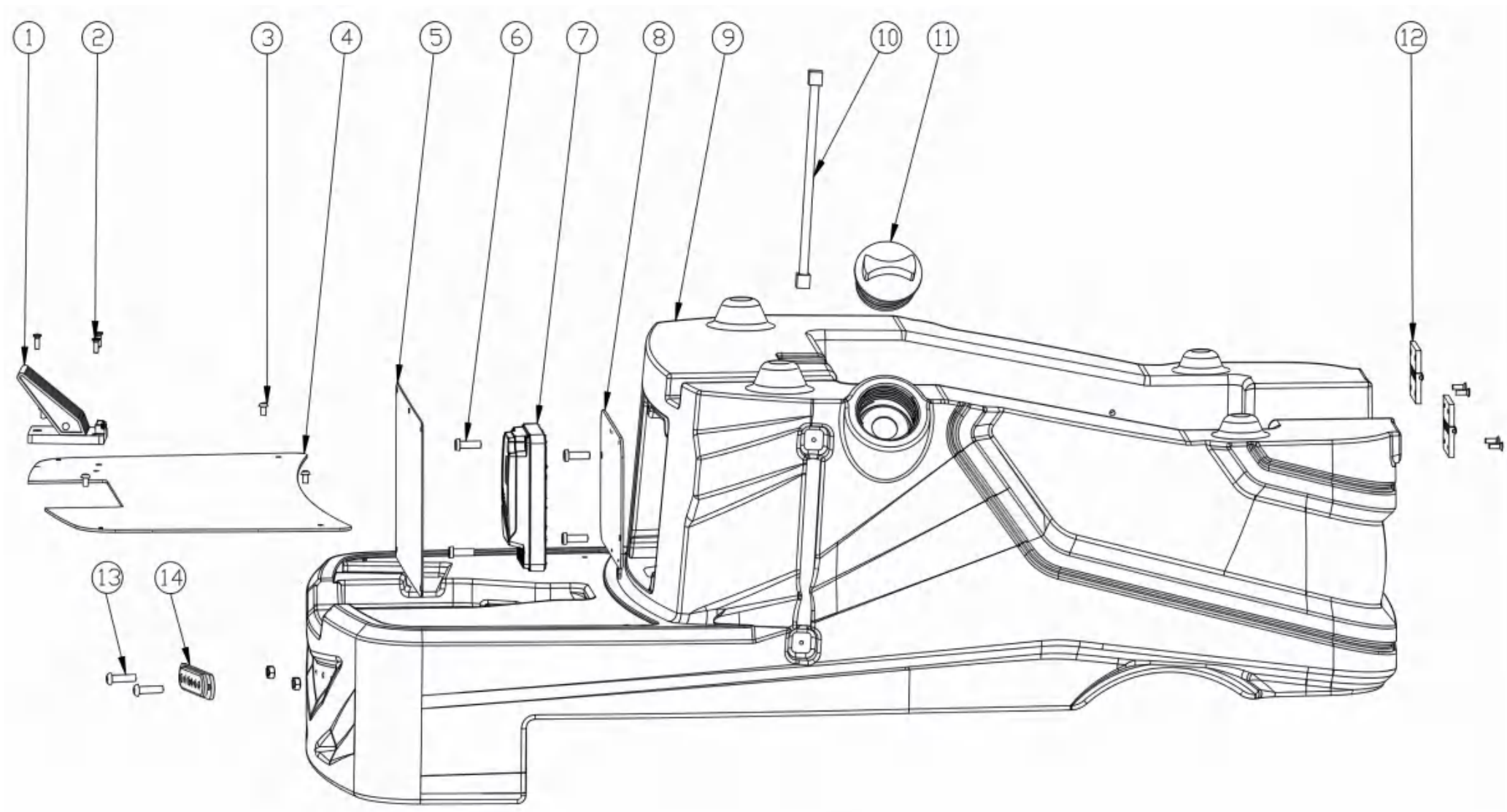
Fig. 2 -SOLUTION TANK GROUP
