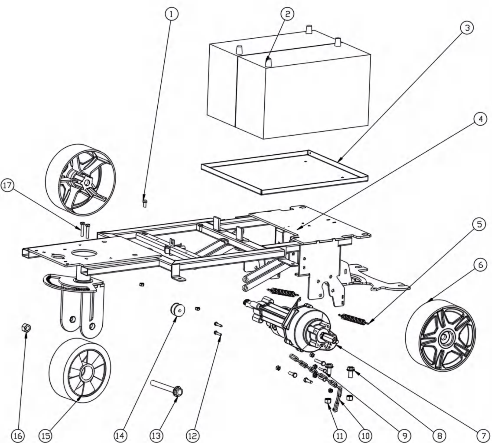
Fig. 4 -MAIN FRAME GROUP
